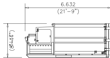
Ultimate - 32yd Demountable Compactor
